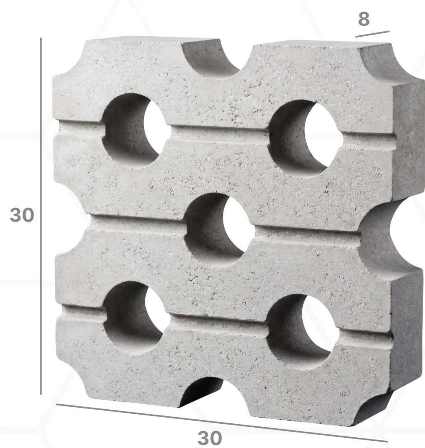
GRASS BLOCK 8 CM
