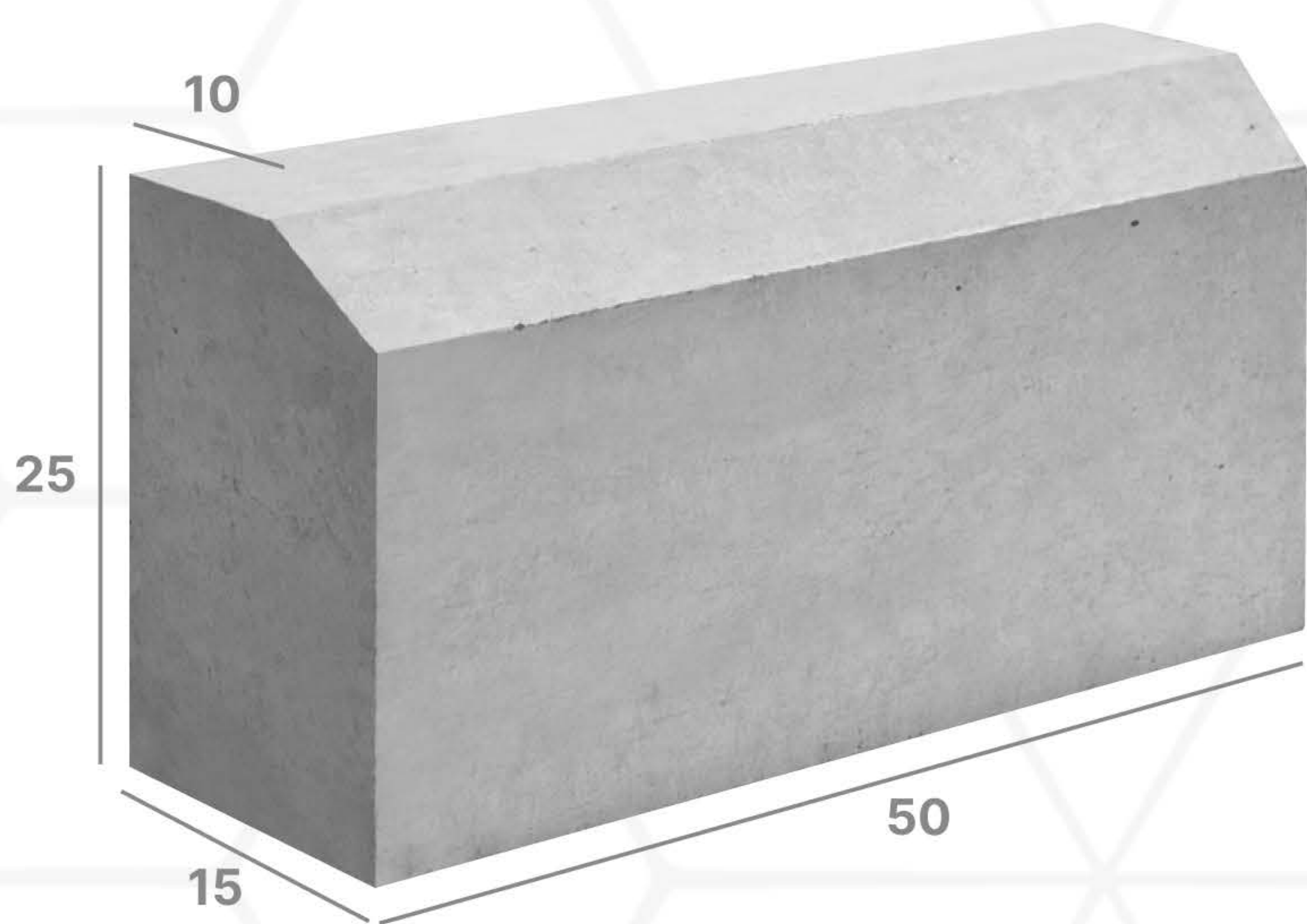
PAVING TAMAN
