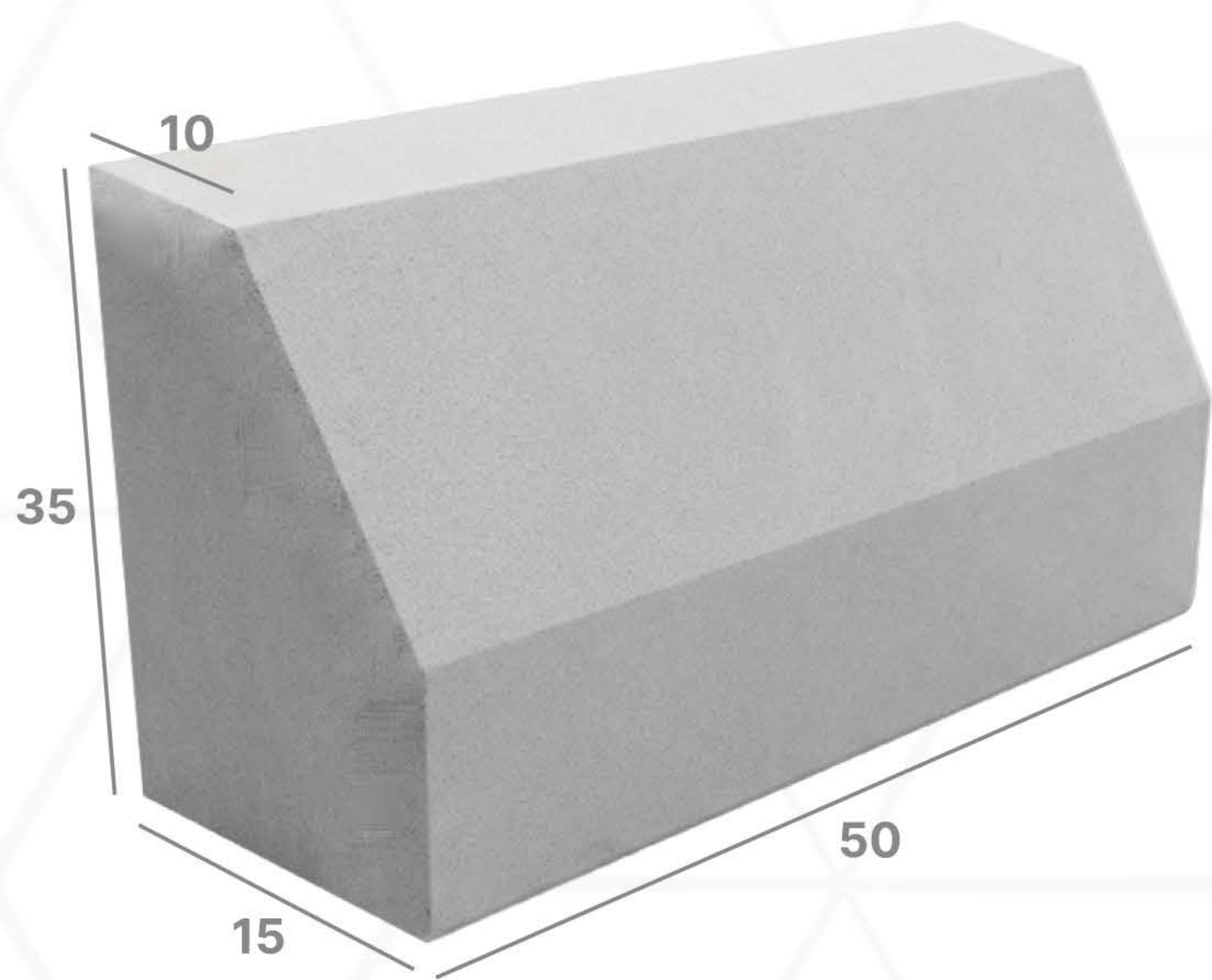
PAVING KANSTIN DKI 1
