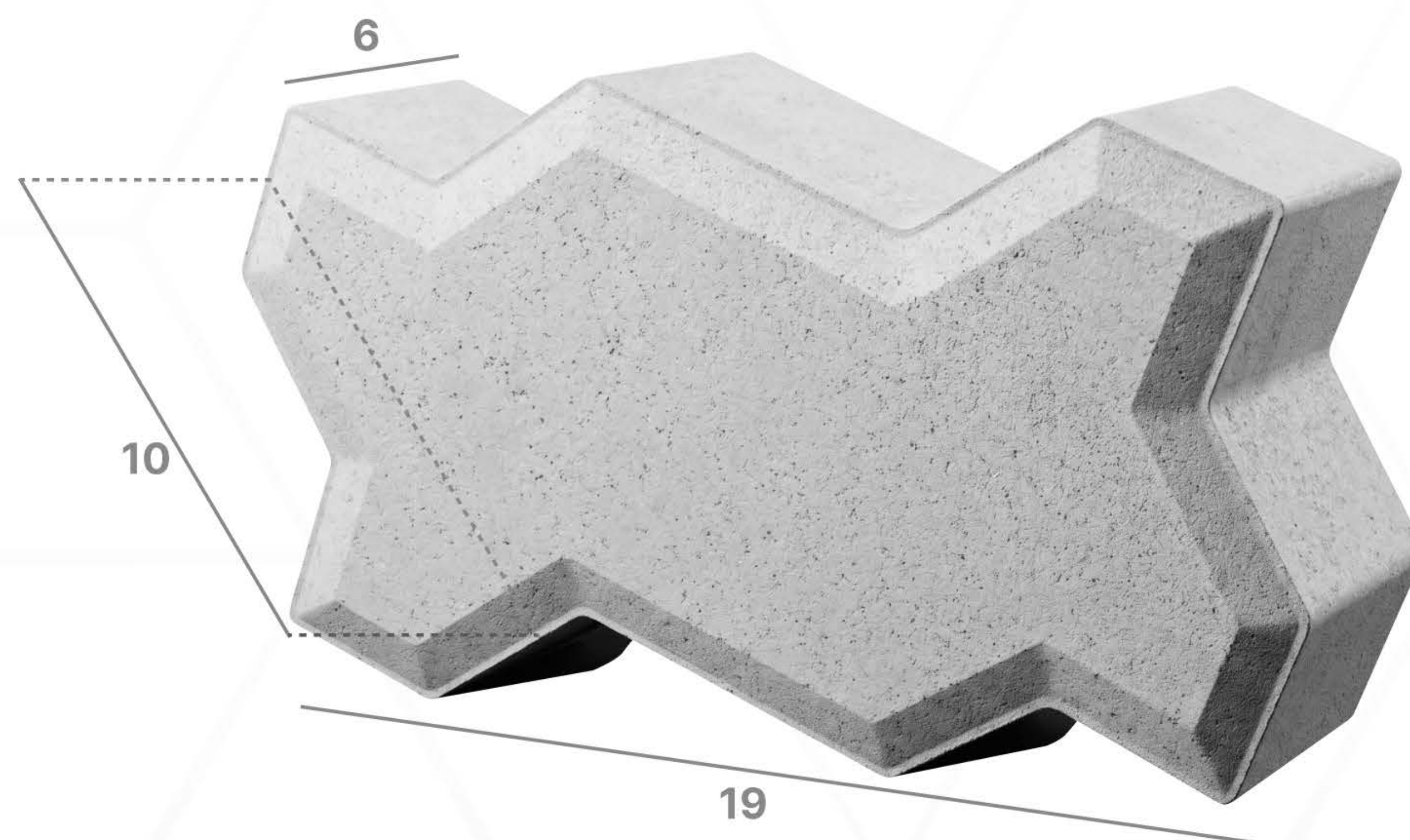
UNI PAVE / CACING 6 CM
