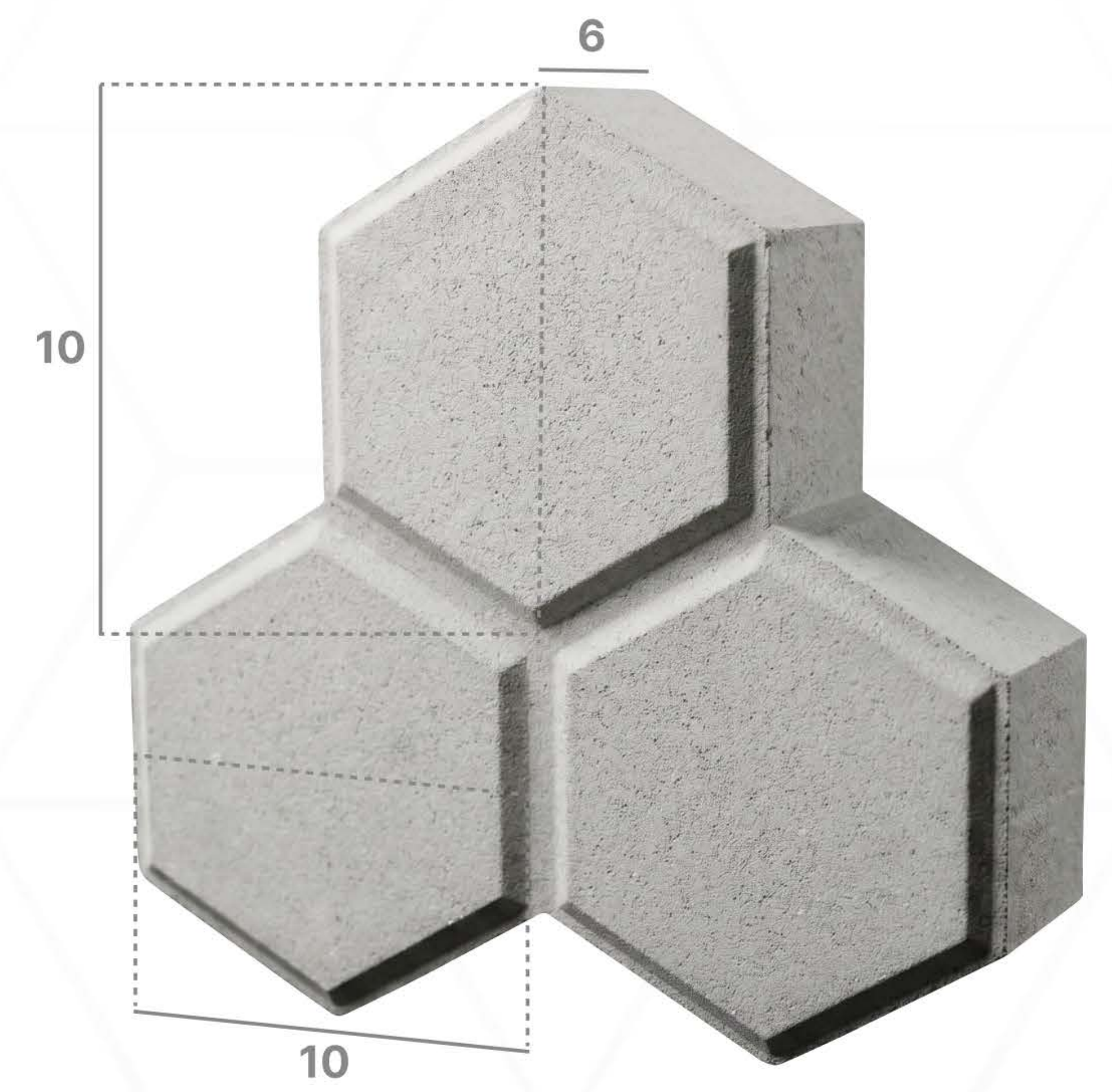
TIGA BERLIAN 6 CM
