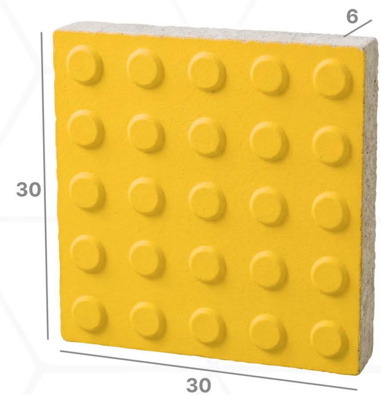
GUIDING BLOCK 6 CM
